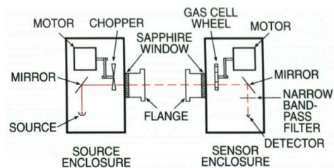
Infrared Analyzer
