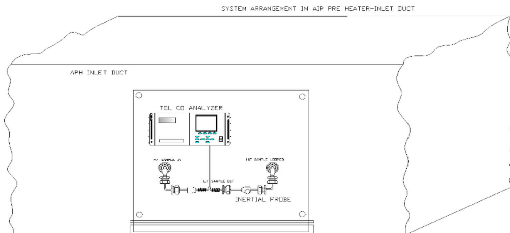
Model TDL 24 General Layout
